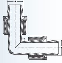
DAMLAMA DİRSEK Dripline Elbow
